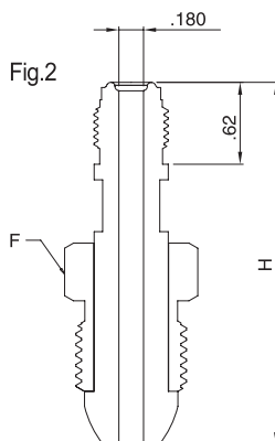
Faceseal Male
