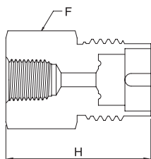
NPT Female
